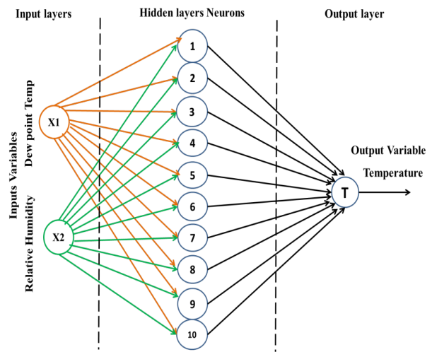
Fig. 2. 3 layered Feed-forward neural network
