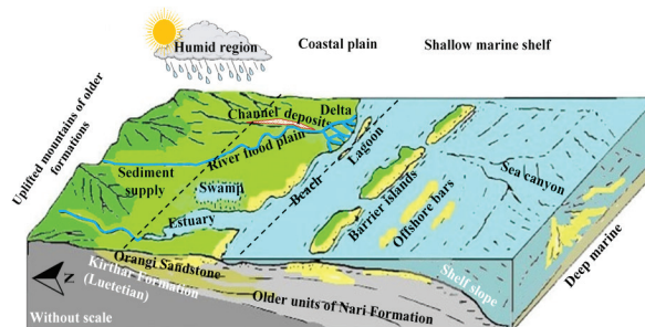
Fig. 13. Hypothetical sketch showing depositional model of Orangi Sandstone in the study area during Oligocene, marked by broken lines.
